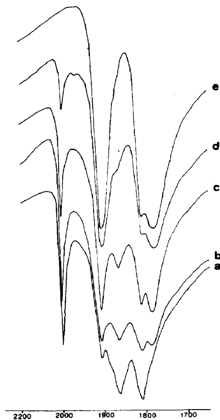
Fig. 1. IR spectra in the \nu(\text{C}\equiv\text{O}) region of the reaction \text{W}(\text{CO})_4(\eta^2\text{-bpy}) with dppm at different times: (a) 15 min; (b) 30 min; (c) 1 h; (d) 1.5h; (e) 2 h.
