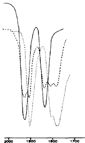
Fig. 2. IR spectra in the \nu(\text{C}\equiv\text{O}) region of \text{W}(\text{CO})_3(\eta^2\text{-bpy})(\eta^1\text{-dppm}) in \text{CHCl}_3 : ..... 4 h at room temperature under \text{N}_2 ; — 4 h at reflux under \text{N}_2 ; - - - - 3 h at reflux under CO.
