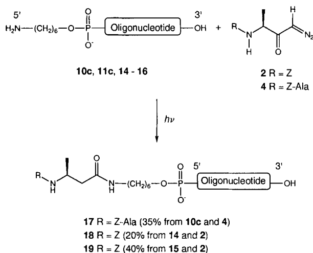
Scheme 4. Diazo-Ketone Decomposition with Wolff Rearrangement and Ketene Trapping by O P5' -Aminoalkyl-Substituted Oligonucleotides 10c , 11c , and 14–16
