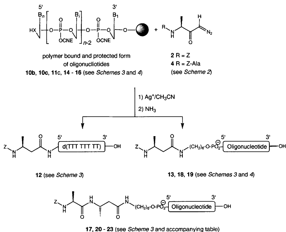
Scheme 5. \text{Ag}^+ -Induced Decomposition of Excess Diazo Ketones 2 and 4 in the Presence of Solid-Support-Bound and Protected Oligonucleotide Derivatives and Cleavage/Deprotection to Give the Conjugates 12 , 13 , and 17–23 a)
