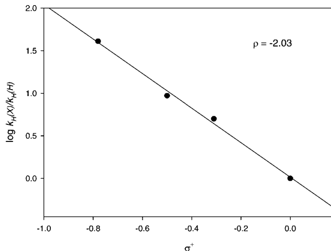
FIGURE 1. Dependence of the \log k_H(X)/k_H(H) for the reactions of N,N -dimethylanilines 1–4 with dp -ph • in CH 3 CN at 25 °C upon the Brown-Okamoto \sigma^+ constants.
