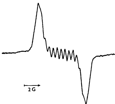
Fig. 5. EPR spectrum of \text{Mn}(\text{CO})_3(\text{bpy}')(p\text{-DBSQ}) generated by 546 nm-irradiation of 10^{-2} M \text{Mn}_2(\text{CO})_8(\text{bpy}') and 2 \times 10^{-2} M p\text{-DBQ} in toluene at 295 K.
