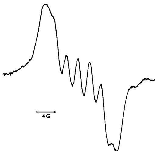
Fig. 9. EPR spectrum of \text{Mn(CO)}_5(\text{O-}o\text{-DBSQ}) generated by 366 nm photolysis of 3.8 \times 10^{-3} \text{ M} \text{Mn}_2(\text{CO})_{10} and 10^{-2} \text{ M} o\text{-DBQ} in toluene at 188 K.
