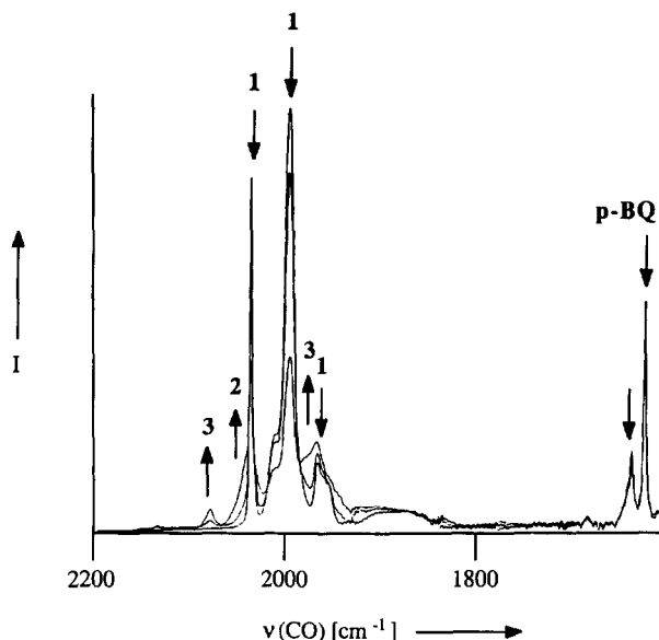
Fig. 2. IR spectral changes upon photolysis of a \text{Mn}_2(\text{CO})_{10}/p\text{-BQ} (1:5) solution in toluene at 220 K with 351/364 nm (20 mW) light. (Bands are labelled as follows: 1 = \text{Mn}_2(\text{CO})_{10} , 2 = \text{Mn}(\text{CO})_5(p\text{-BSQ}) , 3 = \text{Mn}_2(\text{CO})_9(p\text{-BQ}) .)
