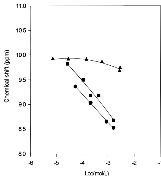
Figure 3. Chemical shift of aromatic protons of zinc phthalocyanines, as a function of log concentration (mol/L). ^1\text{H} NMR in \text{C}_6\text{D}_6 at 27 °C: \blacktriangle , (3,3-dimethylbutynyl) _8\text{PcZn} ( 28 ); \bullet , (hexynyl) _8\text{PcZn} ( 26 ); \blacksquare , (octynyl) _8\text{PcZn} ( 24 ).
