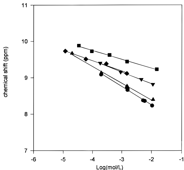
Figure 2. Chemical shift of aromatic protons of metal free phthalocyanines, as a function of log concentration (mol/L). ^1\text{H} NMR in \text{C}_6\text{D}_6 at 27 °C: \blacksquare , (3,3-dimethylbutynyl) _8\text{PcH}_2 ( 23 ); \bullet , (hexynyl) _8\text{PcH}_2 ( 21 ); \blacktriangle , (heptynyl) _8\text{PcH}_2 ( 20 ). ^1\text{H} NMR in \text{CDCl}_3 at 27 °C: \blacktriangledown , (3,3-dimethylbutynyl) _8\text{PcH}_2 ( 23 ). ^1\text{H} NMR in nitrobenzene- d_5 at 27 °C: \blacksquare , (3,3-dimethylbutynyl) _8\text{PcH}_2 ( 23 ).
