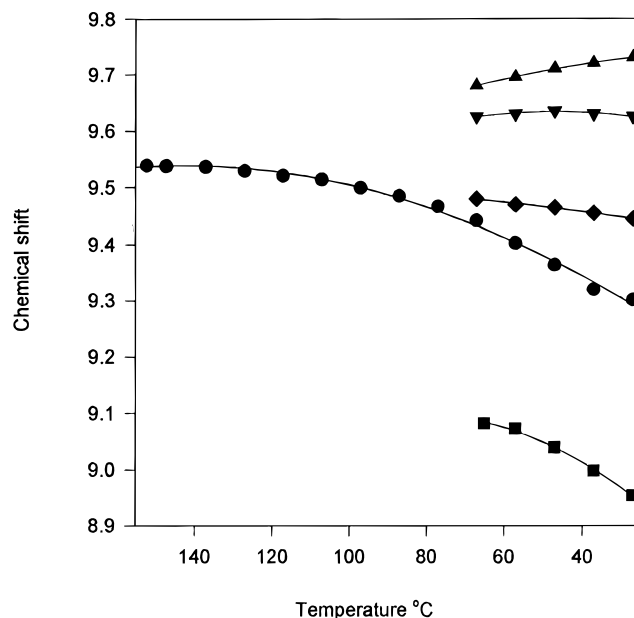
Figure 4. Dependence on temperature of the chemical shift of aromatic protons of metal-free (3,3-dimethylbutynyl) _8\text{PcH}_2 ( 23 ): \bullet , in nitrobenzene- d_5 ( 1.1 \times 10^{-3} M); \blacksquare , in \text{CDCl}_3 ( 3.6 \times 10^{-3} ). In \text{C}_6\text{D}_6 : \blacklozenge , 1.5 \times 10^{-3} ; \blacktriangledown , 4.0 \times 10^{-4} ; \blacktriangle , 9.4 \times 10^{-5} mol/L.
