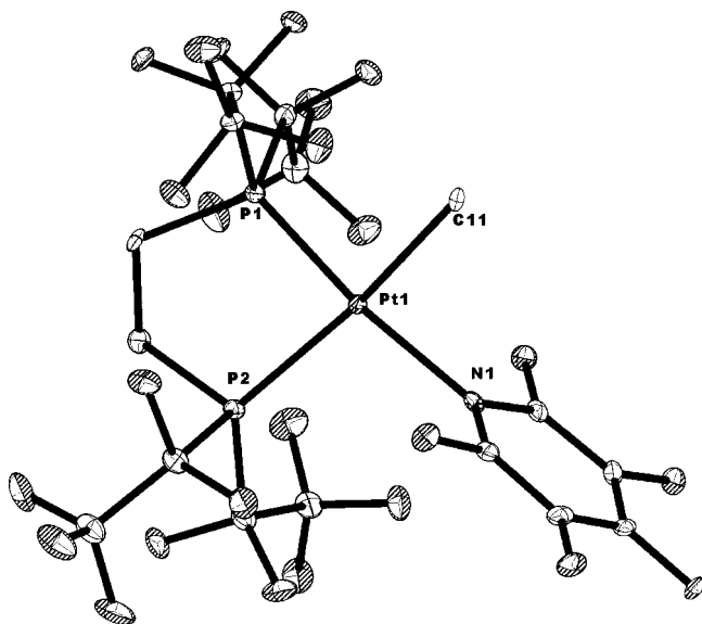
Figure 3. Molecular structure of [(dfepe)Pt(Me)(NC 5 F 5 )] + B(C 6 F 5 ) 4 − ( 5 ) (borate anion and hydrogen atoms are omitted for clarity) with atom-labeling scheme (ellipsoids are drawn at 30% probability). Selected metrical data (Å, deg): Pt(1)–P(1) 2.1747(10); Pt(1)–P(2) 2.3294(11); Pt(1)–C(11) 2.080(4); Pt(1)–N(1) 2.153(4); C(11)–Pt(1)–N(1) 85.40(14).
