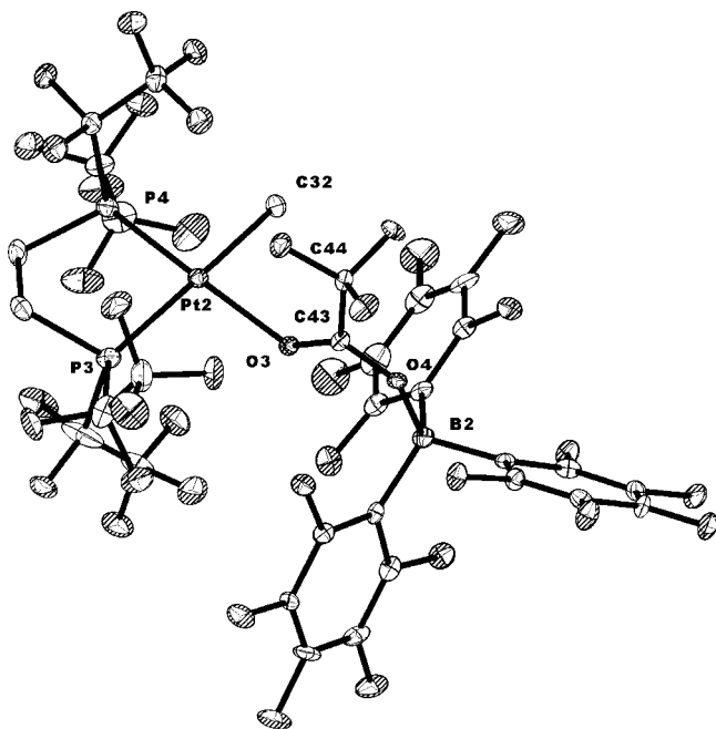
Figure 1. Molecular structure of (dfepe)Pt(Me)(O 2 CCF 3 )B(C 6 F 5 ) 3 ( 2 ) (hydrogen atoms are omitted for clarity) with atom-labeling scheme (ellipsoids are drawn at 30% probability; only the Pt(2) unit with its associated atoms is shown). Selected metrical data (Å, deg): Pt(2)–P(3) 2.314(2); Pt(2)–P(4) 2.161(2); Pt(2)–O(3) 2.115(5); Pt(2)–C(32) 2.084(7); O(3)–C(43) 1.245(9); C(43)–O(4) 1.258(9); O(4)–B(2) 1.571(10); C(32)–Pt(2)–O(3) 85.4(3); P(3)–Pt(2)–P(4) 85.57(8); C(43)–O(3)–Pt(2) 133.5(5); O(3)–C(43)–O(4) 126.4(7); C(43)–O(4)–B(2) 127.6(6).
