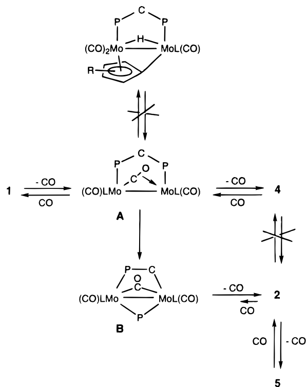
Scheme 1. Proposed Reaction Pathways in the Decarbonylation Reactions of Compounds 1 a
