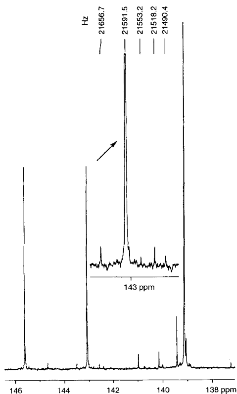
Fig. 3. ^1H -Decoupled ^{13}C -NMR spectrum (150.904 MHz; CDCl_3 ) of the isotopically isomeric mixture of [^{13}C_2] - 6a : range of C(6), C(5), C(10), and C(3). The insert shows the enhanced signal of C(5).
