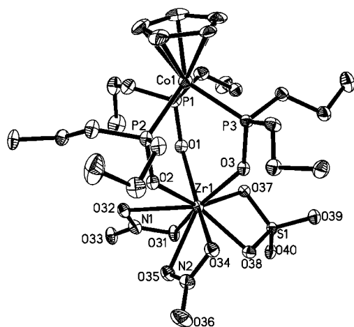
Figure 8. Molecular structure of the anion [(L_{OEt})_2Zr(NO_3)_2(SO_4)]^- in 10 . The ellipsoids are drawn at 30% probability level. Selected bond lengths [Å] and angles [°]: Zr1–O( L_{OEt} ) 2.114(3)–2.175(4), Zr1–O31 2.300(3), Zr1–O32 2.439(4), Zr1–O34 2.403(4), Zr1–O35 2.294(4), Zr1–O37 2.232(3), Zr1–O38 2.164(4), O31–N1 1.289(6), O32–N1 1.269(6), O33–N1 1.219(5), O35–N2 1.292(6), O36–N2 1.205(6), S1–O37 1.499(4), S1–O38 1.521(4), S1–O39 1.437(4), S1–O40 1.438(4), O31–Zr1–O32 53.98(13), O35–Zr1–O34 54.04(13), O38–Zr1–O37 62.77(13).
