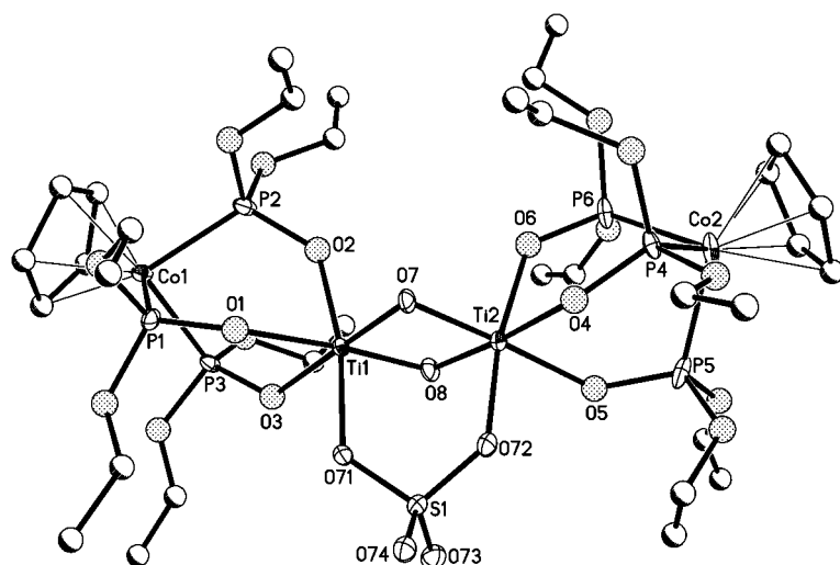
Figure 1. Molecular structure of 2 . The ellipsoids are drawn at 30% probability level. Selected bond lengths [Å] and angles [°]: Ti–O( L_{OEt} ) 1.971(4)–2.118(4), Ti1–O7 1.797(4), Ti1–O8 1.845(4), Ti2–O7 1.862(4), Ti2–O8 1.819(4), Ti1–O71 1.994(4), Ti2–O72 1.977(4), Ti1–Ti2 2.7050(13), S1–O71 1.523(4), S1–O72 1.524(5), S1–O73 1.438(5), S1–O74 1.427(5); Ti1–O7–Ti2 95.3(2), Ti1–O8–Ti2 95.2(2), Ti1–O71–S1 127.6(3), Ti2–O72–S1 128.3(3).
