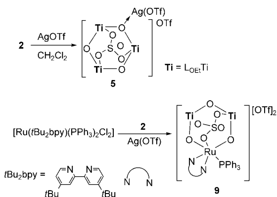
Scheme 2. Preparations of trinuclear Ti sulfato complexes 5 and 9 .
