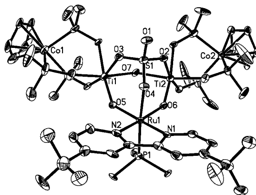
Figure 6. Molecular structure of the dication [(\text{L}_{\text{OEt}})_2\text{Ti}_2(\mu\text{-O})](\mu_3\text{-SO}_4)(\mu\text{-O})_2\{\text{Ru}(\text{PPh}_3)(\text{tBu}_2\text{bpy})\}]^{2+} in 9 . The ellipsoids are drawn at 30 % probability level. Ethyl groups in \text{L}_{\text{OEt}} and phenyl ring in the \text{PPh}_3 are omitted for clarity. Selected bond lengths [Å] and angles [°]: Ru1–N1 2.049(7), Ru1–N2 2.048(7), Ru1–O4 2.163(5), Ru1–O5 1.973(6), Ru1–O6 1.975(5), Ru1–P1 2.302(2), Ti1–O( \text{L}_{\text{OEt}} ) 1.959(6)–2.103(6), Ti1–O3 2.029(6), Ti1–O5 1.732(5), Ti1–O7 2.009(6), Ti2–O2 2.032(6), Ti2–O6 1.719(6), Ti2–O7 2.040(6), S1–O1 1.431(6), S1–O2 1.488(6), S1–O3 1.491(6), S1–O4 1.485(6); O5–Ru1–P1 93.90(18), O6–Ru1–P1 91.45(17), N2–Ru1–P1 95.9(2), N1–Ru1–P1 92.6(2), O4–Ru1–P1 174.98(17), Ti1–O5–Ru1 138.5(3), Ti2–O6–Ru1 140.2(3), Ti1–O7–Ti2 130.8(3).
