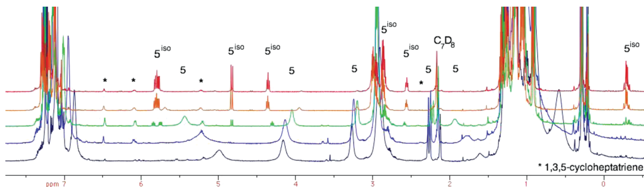
Figure 5. Stacked plot of the ^1\text{H} NMR spectra recorded in \text{C}_7\text{D}_8 illustrating the isomerization of 5 to 5 iso with the appearance of free CHT (*). Bottom to top: 313, 333, 353, 373, and 373 K after 10 min.
