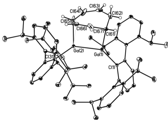
Figure 6. Thermal ellipsoid (30%) plot of S^{iso} . Ligand H atoms and a cocrystallized diethyl ether solvent molecule are not shown. Selected bond lengths (Å) and angles (deg): Ga(1)–Ga(2), 2.469(3); Ga(1)–C(1), 1.985(2); Ga(2)–C(31), 1.983(6); Ga(1)–C(61), 2.020(7); Ga(2)–C(65), 2.219(4); Ga(2)–C(66), 2.352(3); C(61)–C(62), 1.507(3); C(62)–C(63), 1.447(3); C(63)–C(64), 1.367(3); C(64)–C(65), 1.479(4); C(65)–C(66), 1.398(4); C(66)–C(67), 1.337(4); C(67)–C(61), 1.494(3); C(1)–Ga(1)–Ga(2), 136.48(4), C(1)–Ga(1)–C(61), 128.89(6); C(31)–Ga(2)–Ga(1), 138.13(5); C(31)–Ga(2)–C(65), 123.98(7); Ga(1)–Ga(2)–C(65), 97.18(6); Ga(2)–Ga(1)–C(61), 118.09(14).
