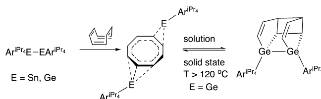
Scheme 1. Reactions of COT with \text{Ar}^{\text{iPr}_4}\text{EEAr}^{\text{iPr}_4} ( \text{E} = \text{Sn} , 6 \text{Ge} ) 7
