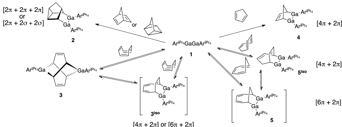
Scheme 2. Cycloadditions of Various Polyolefins with \text{Ar}^{\text{iPr}_4}\text{GaGaAr}^{\text{iPr}_4} ( 1 )
