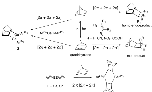
Scheme 3. Reactions of NBD and Quadricyclane with \text{Ar}^{\text{iPr}_4}\text{EEAr}^{\text{iPr}_4} ( \text{E} = \text{Ga}, \text{Ge}, \text{Sn} ) and Other Dienophiles ( \text{R} = \text{H} or Electron-Withdrawing Group, e.g., CN or COOR)
