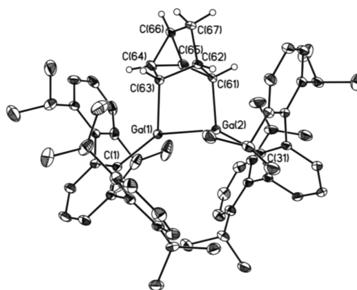
Figure 1. Thermal ellipsoid (30% probability) plot of 2 . Selected H atoms, a crystallographically independent deltacyclane molecule, and a cocrystallized hexane molecule are not shown. Selected bond lengths (Å) and angles (deg): Ga(1)–Ga(2), 2.470(4); Ga(1)–C(1), 1.990(2); Ga(2)–C(31), 1.983(3); Ga(1)–C(63), 2.081(4); Ga(2)–C(61), 2.037(4); C(61)–C(62), 1.570(6); C(61)–C(65), 1.514(5); C(62)–C(63), 1.573(6); C(62)–C(67), 1.514(7); C(65)–C(66), 1.501(8); C(66)–C(67), 1.483(6); C(1)–Ga(1)–Ga(2), 141.66(4); C(1)–Ga(1)–C(63), 129.21(1); Ga(2)–Ga(1)–C(63), 87.80(12); C(31)–Ga(2)–Ga(1), 141.78(4); C(31)–Ga(2)–C(61), 121.8(12); C(61)–Ga(2)–Ga(1), 90.47(11).
