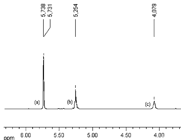
Figure 3. ^1\text{H} NMR spectrum of 7a in \text{CDCl}_3/\text{acetone-}d_6 : (a) Cp; (b) free 18:1; (c) coordinated 18:1.
