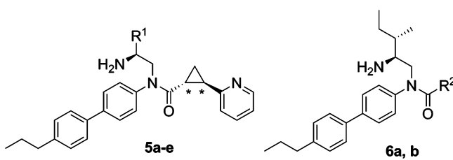
5a–e 6a, b *(R, R) and (S, S) mixture
