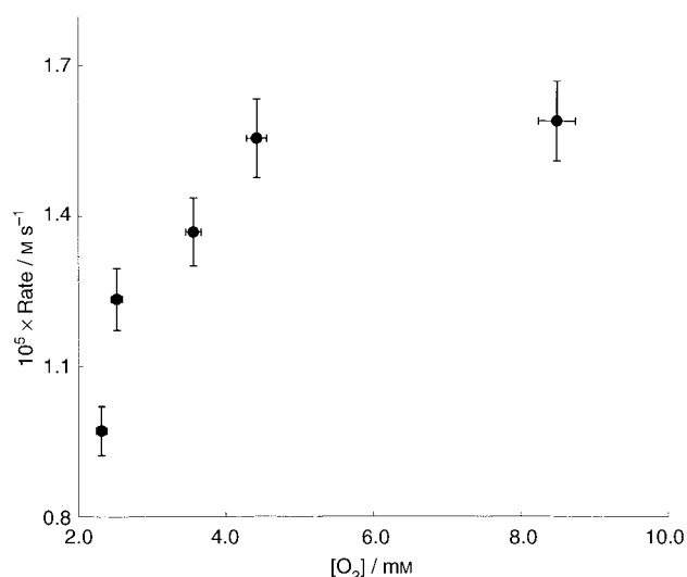
Figure 1. Rate of p -cymene formation in acetonitrile at 50°C with [TH] = 0.428 M and [AIBN] = 5.09 \times 10^{-3} M at various oxygen concentrations.
