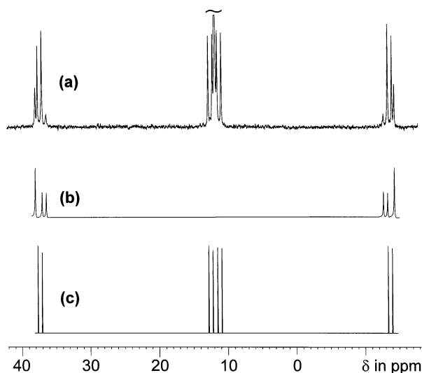
Fig. 1. Experimental (a) and simulated (b, c) ^{31}\text{P} -NMR spectra of [\{\text{PtCl}_2(\text{C}_4\text{Me}_4)\}_2(\mu\text{-Ph}_2\text{PCH}_2\text{PPh}_2)] ( 2b ). The spectra b (AA' part of the AA'XX' subspectrum) and c (AB part of the ABX subspectrum; A, B = ^{31}\text{P} ; X = ^{195}\text{Pt} ) were separately calculated and are shown in the approximate ratio of their abundances (44.8% : 11.4%).
