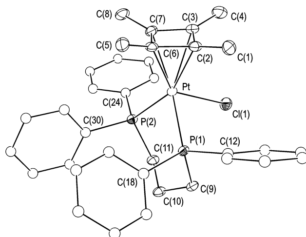
Fig. 3. ORTEP-III plot of the molecular structure of the cation in [\text{PtCl}(\text{C}_4\text{Me}_4)\{\text{Ph}_2\text{P}(\text{CH}_2)_3\text{PPh}_2\}]\text{Cl}\cdot\text{CH}_2\text{Cl}_2 ( 5b · \text{CH}_2\text{Cl}_2 ), 30% displacement ellipsoids.
