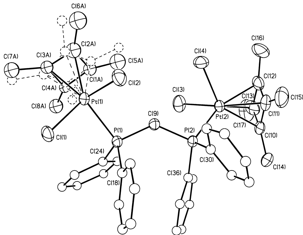
Fig. 2. ORTEP-III plot [16] of the molecular structure of [\{\text{PtCl}_2(\text{C}_4\text{Me}_4)\}_2(\mu\text{-Ph}_2\text{PCH}_2\text{PPh}_2)] ( 2b ), 40% displacement ellipsoids. Second position of disordered cyclobutadiene ring on Pt(1) is displayed as dashed lines.
