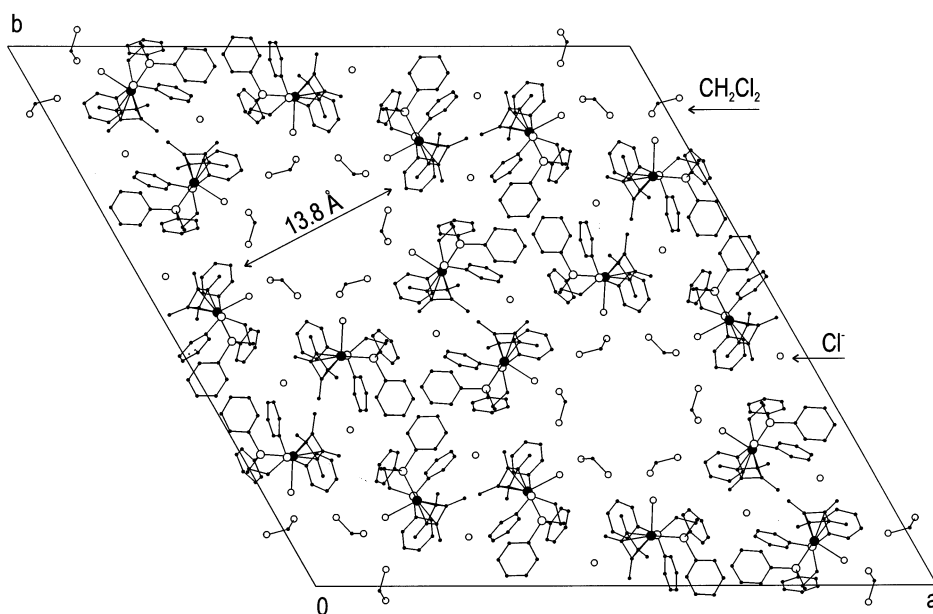
Fig. 4. View of the unit cell of [PtCl(C 4 Me 4 ){Ph 2 P(CH 2 ) 3 PPh 2 )]Cl·CH 2 Cl 2 ( 5b ·CH 2 Cl 2 ) along the c -axis, only the major (70%) position of the solvate molecule is displayed.
