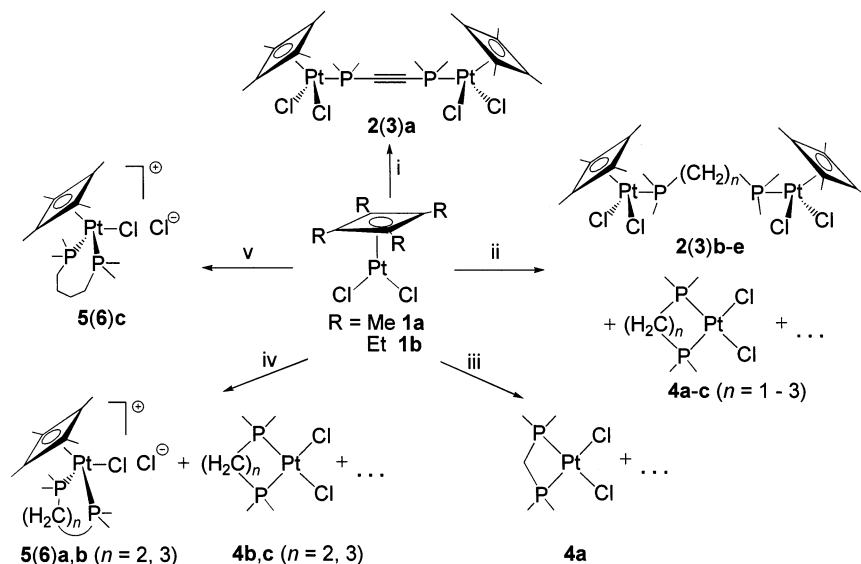
Scheme 1. i) dp pa (2:1); ii) dp pm, dp pe, dp pp, dp pb (2:1); iii) dp pm (1:1); iv) dp pe, dp pp (1:1); v) dp pb (1:1).
