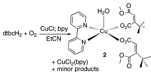
Scheme 2. The Formation of Complex 2
