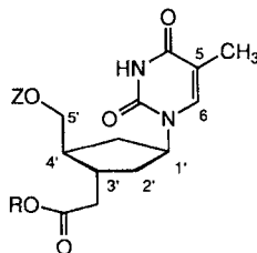
2a Z = ( t -Bu)Me 2 Si, R = PhCH 2 2) b Z = H, R = PhCH 2 2)
