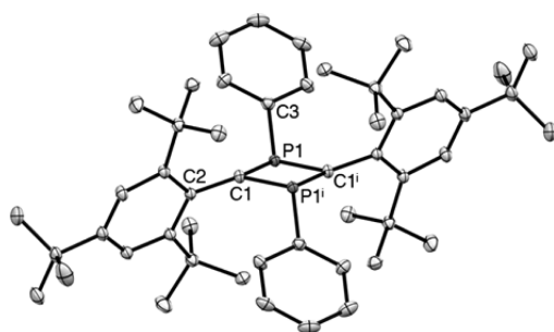
Figure 7. ORTEP drawing for the X-ray structure of 7 (50% probability levels). Hydrogen atoms are omitted for clarity. Selected bond lengths (Å) and angles (deg): P1–C1, 1.7463(2); P1'–C1, 1.7502(2); C1–C2, 1.4883(3); P1–C3, 1.8055(3); C1–P1–C1', 93.12(2); C1–P1–C3, 121.88(1); C3–P1–C1', 117.78(1); P1–C1–P1', 86.88(1); P1–C1–C2, 139.55(2); P1'–C1–C2, 129.54(2) (superscript "i" indicates symmetry code 1 - x, 1 - y, 1 - z ).
