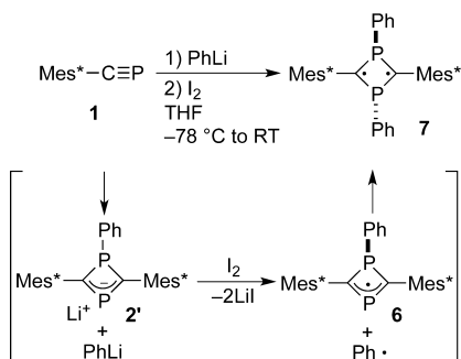
Scheme 4. SET-Based Preparation of 7 from 1 through Intermediates 2' and 6
