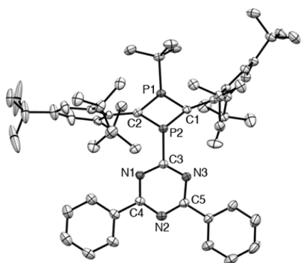
Figure 3. ORTEP drawing of the molecular structure of 5b (40% probability levels). Hydrogen atoms and the solvent molecule (dichloromethane) are omitted for clarity. The 4-C( t Bu) group is disordered, and the atoms of higher occupancy factor (0.58) are shown.
