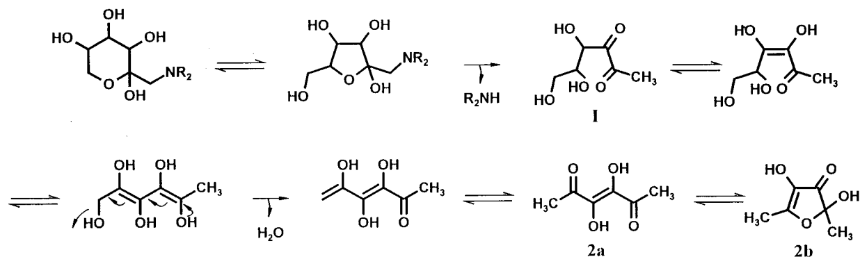
Figure 2. Formation of acetylformoin [3,4-dihydroxy-3-hexene-2,5-dione ( 2a ) and 2,4-dihydroxy-2,5-dimethyl-3(2H)-furanone ( 2b )] via 1-deoxy-2,3-hexodiolose as the key intermediate.
