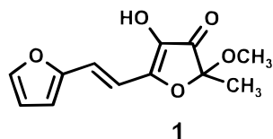
Figure 1. Structure of the yellow 4-hydroxy-2-methoxy-2-methyl-5-[( E )-(2-furyl)methylidene]methyl-2H-furan-3-one ( 1 ).
