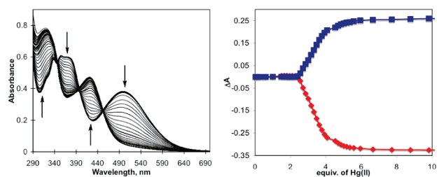
Figure 1. Left: Absorption spectral changes of Pt3 ( 2.0 \times 10^{-5} M) upon the addition of \text{Hg}(\text{ClO}_4)_2 [ (0-1.4) \times 10^{-3} M] in DMF. Right: Changes of absorbance at 500 nm (red curve) and 422 nm (blue curve) versus equivalents of \text{Hg}^{2+} addition.
