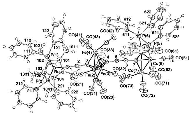
Figure 5. Projection of a molecule of \{\text{Cp}^*(\text{dppe})\text{Ru}\}\text{C}\equiv\text{CC}[\text{Fe}_3(\text{CO})_9]\text{--CC}\equiv\text{CCo}_3(\mu\text{-dppm})(\text{CO})_7 ( 8 ) in 8 · 2\text{C}_6\text{H}_6 .
