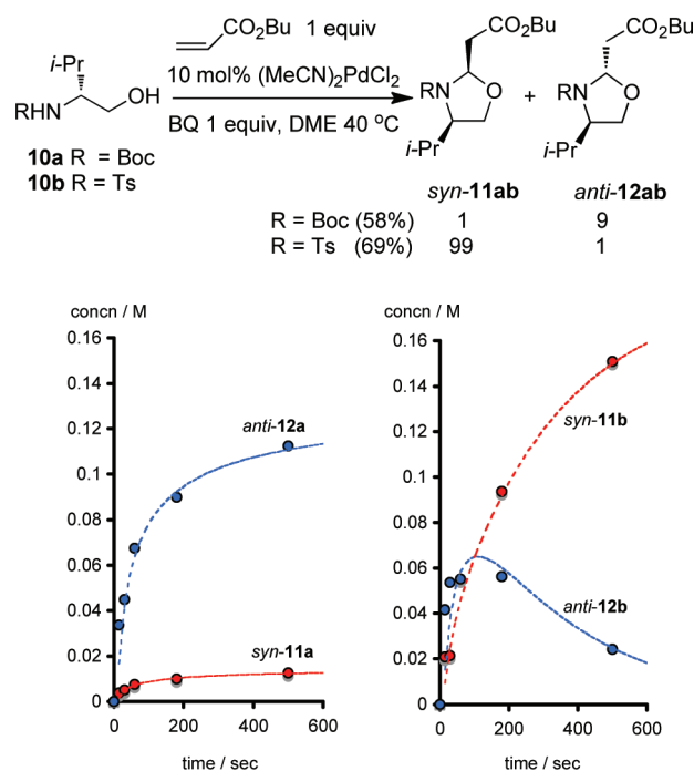
Figure 1. Oxyamination with N -L-valinol derivatives.
