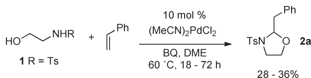
Scheme 1. 2,2-Alkoxyamination of Styrene
