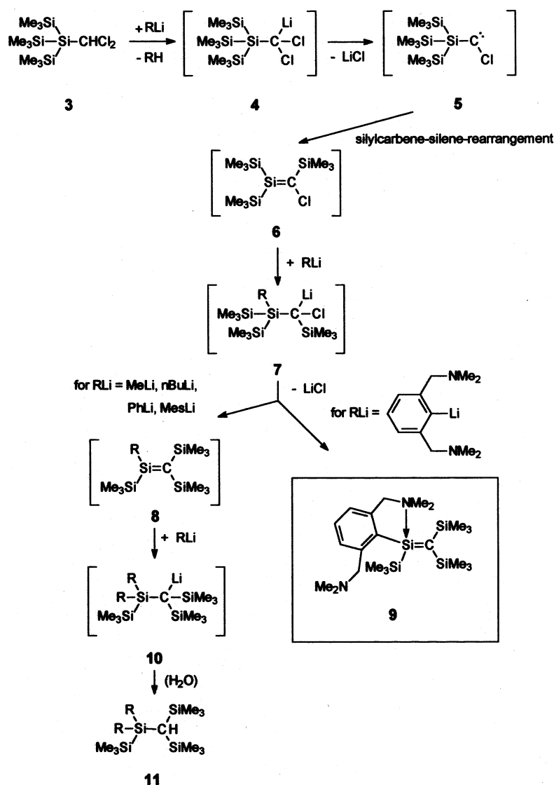
Scheme 1. Reaction of (dichloromethyl)tris(trimethylsilyl)silane ( 3 ) with organolithium reagents RLi, leading in the case of MeLi, n -BuLi, PhLi and MesLi to the congested silanes 11 and affording in the case of 2,6-bis(dimethylaminomethyl)phenyllithium the intramolecularly amine-stabilized silene 9 .
