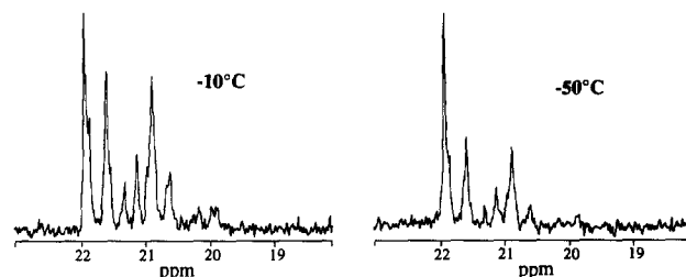
Fig. 2. A comparison of the ^{13}\text{C} NMR methyl pentade resonances of polypropylenes PP4 (prepared with the 11b /methyl alumoxane catalyst at –10°C) and PP6 (–50°C). Spectra in 1,2,4-trichlorobenzene at 350 K.
