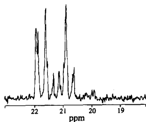
Fig. 1. ^{13}\text{C} NMR methyl pentade signals of polypropylene (PP3) obtained with the 3\beta -5/methylalumoxane catalyst at –50°C (NMR spectrum in 1,2,4-trichlorobenzene at 350 K).
