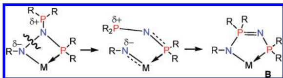
Scheme 3. Proposed Mechanism for the Rearrangement of Diphosphinohydrazides
