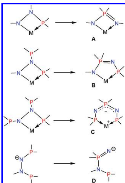
Scheme 1. Rearrangements of Mono-, Bis-, and Triphosphinohydrazides a
