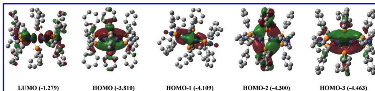
Figure 4. Molecular orbitals for 2 and their energies in electronvolts are provided.
