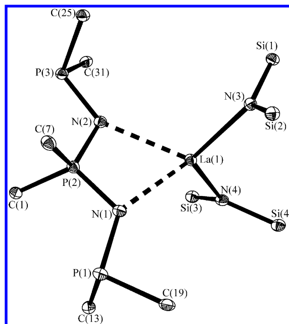
Figure 7. The molecular structure of 5 with ellipsoids of 30% probability. Phenyl and methyl groups and hydrogen atoms were omitted for clarity. Selected bond lengths (Å) and angles (deg) for 5 : \text{La}(1)\text{--N}(3) 2.374(1), \text{La}(1)\text{--N}(4) 2.377(1), \text{La}(1)\text{--N}(1) 2.518(1), \text{La}(1)\text{--N}(2) 2.583(1), \text{P}(2)\text{--N}(1) 1.623(1), \text{P}(2)\text{--N}(2) 1.624(1), \text{P}(1)\text{--N}(1) 1.725(1), \text{P}(3)\text{--N}(2) 1.717(1); \text{N}(3)\text{--La}(1)\text{--N}(4) 116.58(5)^\circ , \text{N}(1)\text{--La}(1)\text{--N}(2) 60.00(4)^\circ , \text{N}(1)\text{--P}(2)\text{--N}(2) 103.59(7)^\circ , \text{P}(1)\text{--N}(1)\text{--P}(2) 115.83(8)^\circ , \text{P}(2)\text{--N}(2)\text{--P}(3) 116.24(8)^\circ .
