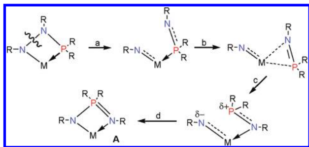
Scheme 3. Proposed Mechanism for the Rearrangement of Diphosphinohydrazides
