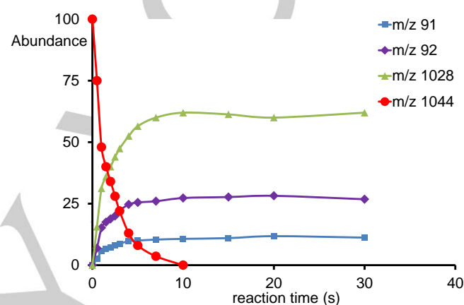
Figure 1. Ion abundances as a function of time after isolation of m/z 1044 ions, i.e. [Fe IV (O)(TPFP + )] + , in the FT-ICR cell in the presence of 5 × 10 -8 mbar cycloheptatriene-7-[D 1 ] at room temperature.
