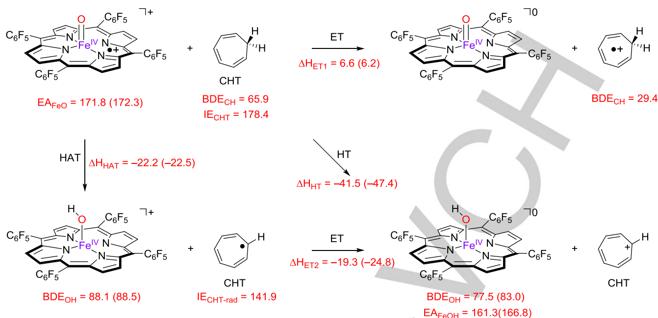
Figure 6. Thermochemical reaction scheme for individual electron, proton and hydride transfer from iron(IV)-oxo and iron(IV)-hydroxo complexes. Data represent reaction enthalpies (in kcal mol -1 ) as calculated at UB3LYP/BS2//UB3LYP/BS1 with ZPE corrections included. Quartet spin data in parenthesis, doublet spin data out of parenthesis.
