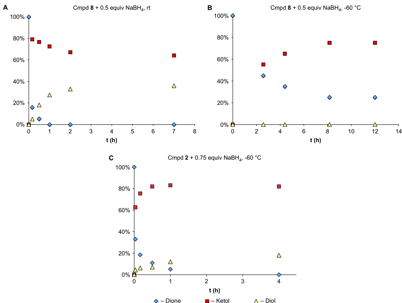
Figure 1. Product distribution analysis over time in the reductions of 8 and 2 with \text{NaBH}_4 in DME.
