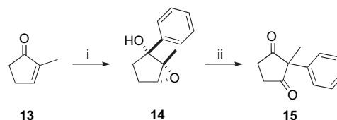
Scheme 2. (i) \text{PhBr} , t\text{-BuLi} (2 equiv), -78\text{ }^\circ\text{C} , then m\text{-CPBA} , DCM, 0\text{ }^\circ\text{C} ; (ii) \text{BF}_3\cdot\text{OEt}_2 , DCM, -40\text{ }^\circ\text{C} , 52% over 3 steps, then \text{PCC} , DCM, 22\text{ }^\circ\text{C} , 1 h, 88%.
