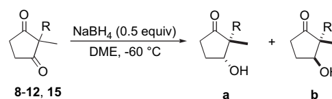
Figure 3. Monoreduction of 2,2-disubstituted-cyclopentane-1,3-diones using 0.5 equiv of \text{NaBH}_4 in DME at -60\text{ }^{\circ}\text{C} .
