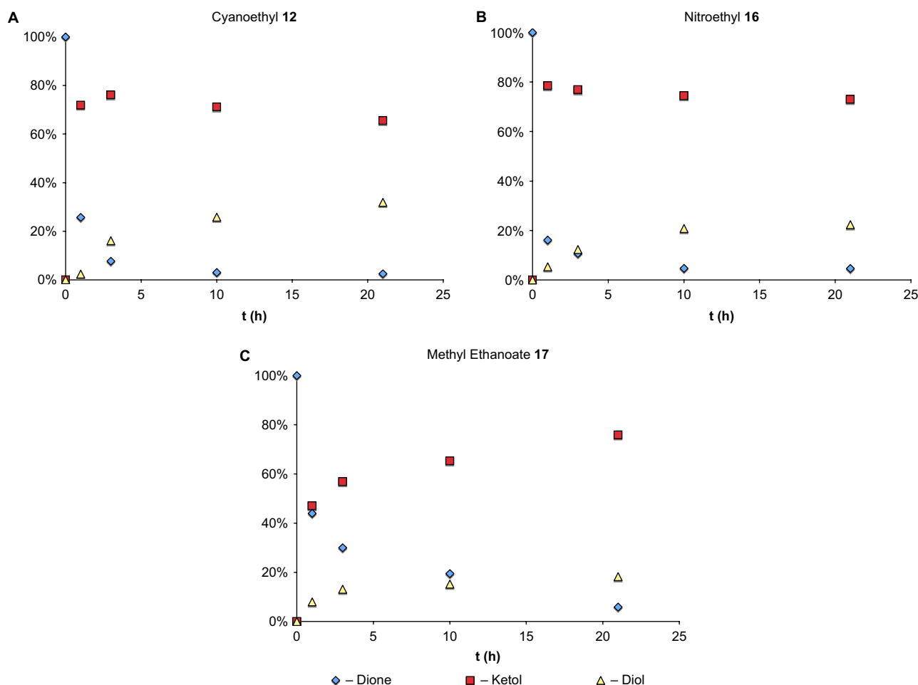
Figure 4. Product distribution analysis over time in the reductions of 12 , 16 , and 17 using NaBH_4 (0.5 equiv) in DME at -60^\circ C .
