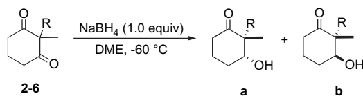
Figure 2. Monoreduction of 2,2-disubstituted-cyclohexane-1,3-diones using 1.0 equiv of \text{NaBH}_4 in DME at -60\text{ }^{\circ}\text{C} .
