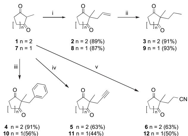
Scheme 1. (i) \text{Pd}(\text{OAc})_2 (cat.), \text{PPh}_3 (cat.), THF, rt, 25 min, then allyl methylcarbonate, rt; (ii) \text{Pd/C} (cat.), \text{H}_2 , rt, 2 h; (iii) \text{LiI} , DBU, MeCN, rt, 1 h, then \text{BnBr} , reflux; (iv) 1 N \text{NaOH} , \text{BrCH}_2\text{CCH} , 60 °C; (v) \text{H}_2\text{CCHCN} , \text{Et}_3\text{N} , reflux.
