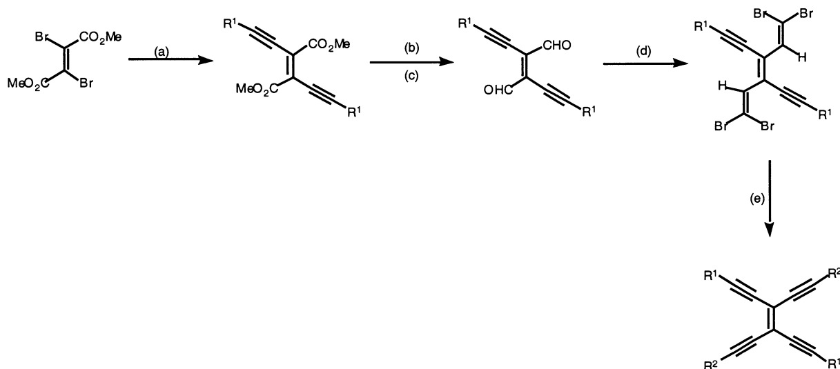
Scheme 2. Synthesis of trans tetraethynylethenes. (a) R 1 C≡CSnBu 3 , PdCl 2 (PPh 3 ) 2 (b) DIBAL-H (c) PCC (d) CBr 4 , Zn, PPh 3 (e) (i) LDA (ii) R 2 -X. DIBAL-H = diisobutylaluminium hydride; PCC = pyridinium chlorochromate; X = halide.
