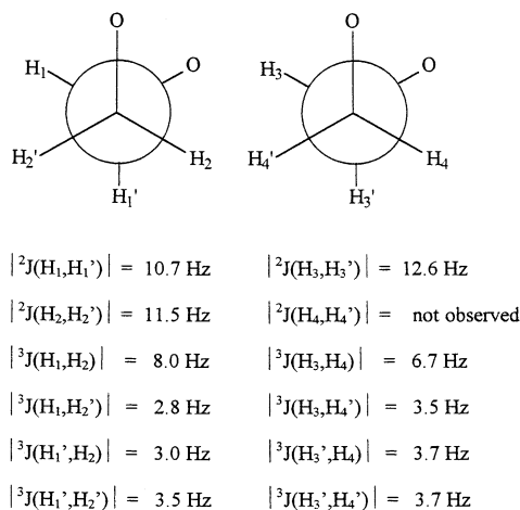
Fig. 3. The magnitudes of geminal |^2J(\text{H,H})| and vicinal coupling constants |^3J(\text{H,H})| of the diastereotopic \text{OCH}_2\text{CH}_2\text{O} fragments of cis -4.
