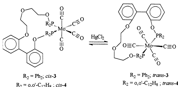
Fig. 6. \text{HgCl}_2 catalyzed cis–trans isomerization of the cis -metallocrown ethers, cis - 3 and cis - 4 .
