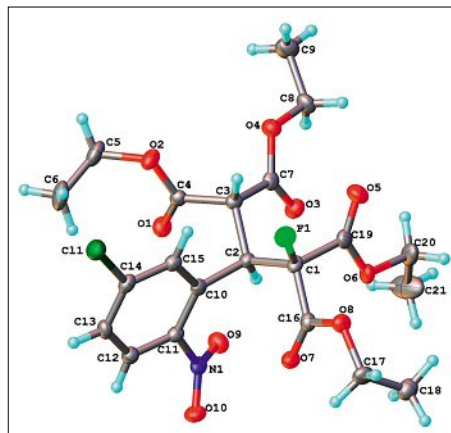
Fig. 2. Molecular structure of one of two independent molecules of 5 .
