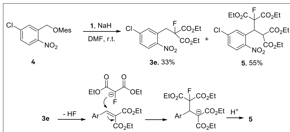
Scheme 2. Reaction of mesylate derivative 4 with 1 .
