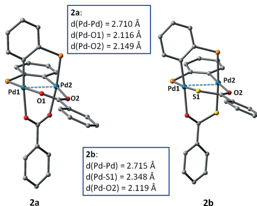
Figure 6. Optimized structures of the \text{Pd}^{\text{II}} carboxylate and thio-carboxylate complexes 2a and 2b . For clarity, hydrogen atoms and free phenyl groups of the phosphine ligands are omitted. Color scheme: Pd green, O red, S yellow, P orange, C gray. The blue dashed lines depict the axial Pd–Pd interactions. The Pd–Pd and Pd–X distances are shown in the boxes.
