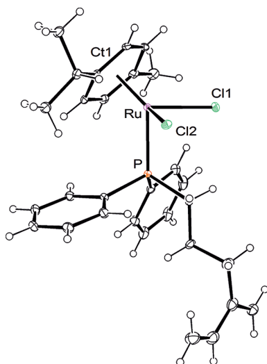
Figure 1. ORTEP view of complex 1 . Selected bonds (Å) and angles ( ^{\circ} ): Ru–Ct1 1.705(10), Ru–Cl1 2.4124(7), Ru–Cl2 2.4203(6), Ru–P 2.3373(6), Ct1–Ru–Cl1 126.08(4), Ct1–Ru–Cl2 127.68(4), Ct1–Ru–P 130.04(4), Cl1–Ru–Cl2 86.15(2), Cl1–Ru–P 88.23(2), Cl2–Ru–P 84.04(2).
