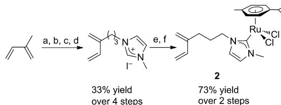
Scheme 2. Synthesis of the arene-ruthenium NHC–diene complex 2 : (a) KDA, ethylene oxide, -80\text{ }^{\circ}\text{C} \rightarrow \text{room temp.} , 3 h; (b) MsCl, \text{NEt}_3 , \text{CH}_2\text{Cl}_2 , room temp., 1 h; (c) imidazole, NaH, THF, room temp., 24 h; (d) \text{CH}_3\text{I} , AcOEt, 3 h, 65\text{ }^{\circ}\text{C} ; (e) \text{Ag}_2\text{O} , \text{CH}_2\text{Cl}_2 , reflux, 24 h; (f) 1/2 [(p\text{-cymene})\text{RuCl}_2]_2 , \text{CH}_2\text{Cl}_2 , room temp., 2 h.
