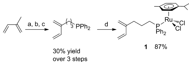
Scheme 1. Synthesis of the arene-ruthenium phosphane–diene complex 1 : (a) KDA, ethylene oxide, -80\text{ }^{\circ}\text{C} \rightarrow \text{room temp.} , 3 h; (b) MsCl, \text{NEt}_3 , \text{CH}_2\text{Cl}_2 , room temp., 1 h; (c) \text{PPh}_2\text{Li} , THF, 0\text{ }^{\circ}\text{C} , 2 h; (d) 1/2 [(p\text{-cymene})\text{RuCl}_2]_2 , benzene, room temp., 4 h.
