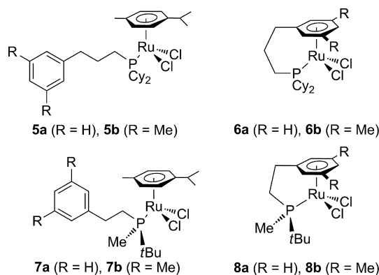
Scheme 5. Structures of non-chelated ( 5 and 7 ) and chelated ( 6 and 8 ) phosphane-arene-ruthenium complexes.
