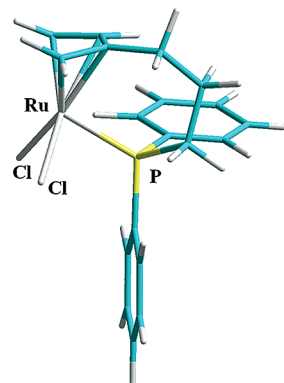
Figure 2. DFT-B3LYP-optimized geometry of [\eta^4\text{-(4-methylenehex-5-enyl)diphenylphosphane-}\kappa\text{P}]\text{RuCl}_2 .
