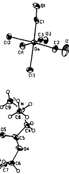
Fig. 3. Molecular structure of 25 in the crystal.
