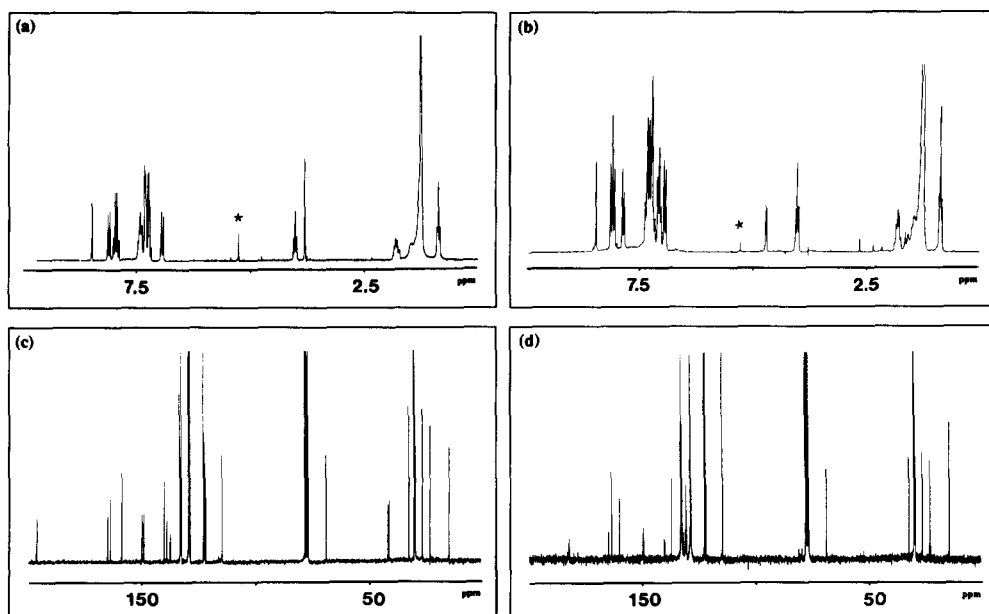
Fig. 1. NMR spectra of compound 8 and complex 14 : (a) ^1\text{H} NMR spectrum of 8 ; (b) ^1\text{H} NMR spectrum of 14 ; (c) ^{13}\text{C}\{^1\text{H}\} NMR spectrum of 8 ; (d) ^{13}\text{C}\{^1\text{H}\} NMR spectrum of 14 . The peaks marked with an asterisk indicate residual \text{CH}_2\text{Cl}_2 .
