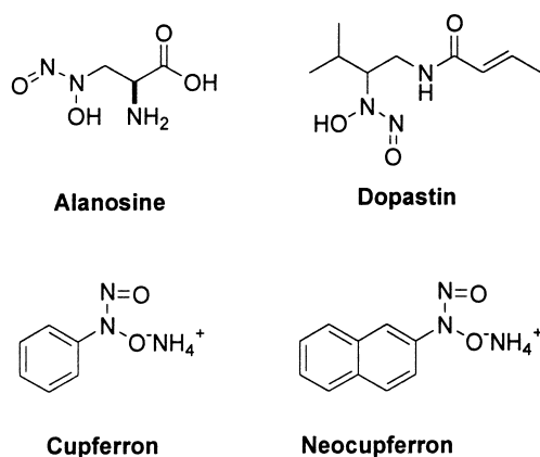
Figure 2. N -Nitroso- N -oxyalkylamines and N -nitroso- N -oxyarylamines.
