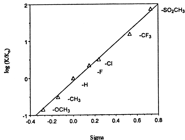
Figure 5. Hammett plot for compounds 1–7 . Equilibrium K and K 0 were calculated as K = e^{(nFE/RT)} . E , the first oxidation potentials, were obtained by cyclic voltammetry experiments (repeated three times) conducted in 1.3 mM solutions of compounds 1–7 in 0.1 M LiClO 4 at pH 7 (adjusted with NH 4 OH and HCl solutions) and at a scan rate of 20 mV/s. R 2 = 0.995.
