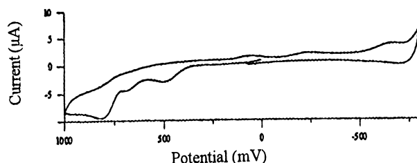
Figure 4. A typical cyclic voltammetry diagram of electrochemical oxidation of compound 1 . Measurements were conducted in 0.1 M LiClO 4 solution with 1.33–1.36 mM of compound at pH 7 (adjusted with NH 4 OH and HCl solutions). The scan rate was 20 mV/s starting at 0 mV with sweeps in three segments, first oxidatively then reductively then oxidatively.
