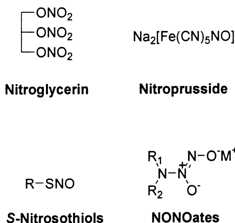
Figure 1. Commonly used NO donor compounds.
