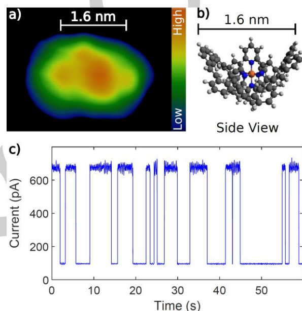
Figure 5. a) Constant-current STM topograph of 1 on Au(111). Current I = 5 pA and sample voltage V = -0.5 V. (b) Side-view model of 1 . Orange, blue, dark gray and light gray spheres represent iron, nitrogen, carbon and hydrogen atoms, respectively. (c) Time series of the tunneling current measured at V = 0.9 V with the tip position frozen over the center of 1 .
