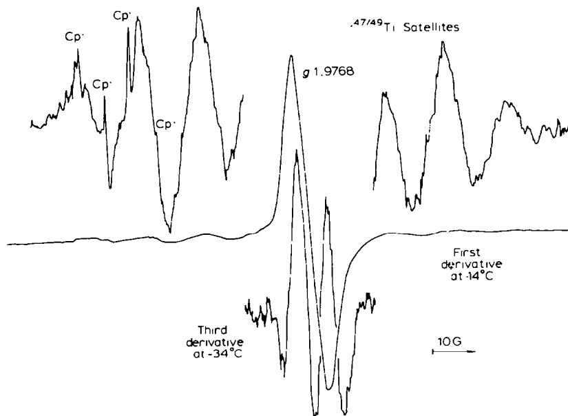
Fig. 2. ESR spectrum from the photolysis of \text{Cp}_2\text{TiCl}_2 in tetrahydrofuran at -14^\circ\text{C} (first derivative) and at -34^\circ\text{C} (third derivative). The upper insets show at higher gain, the ^{47/49}\text{Ti} satellites in the former spectrum, and the central lines of the spectrum of the cyclopentadienyl ( \text{Cp}^\bullet ) radical.
