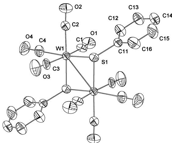
Fig. 1. The structure of [\text{W}_2(\text{SPh})_2(\text{CO})_8] ( 1 ).
