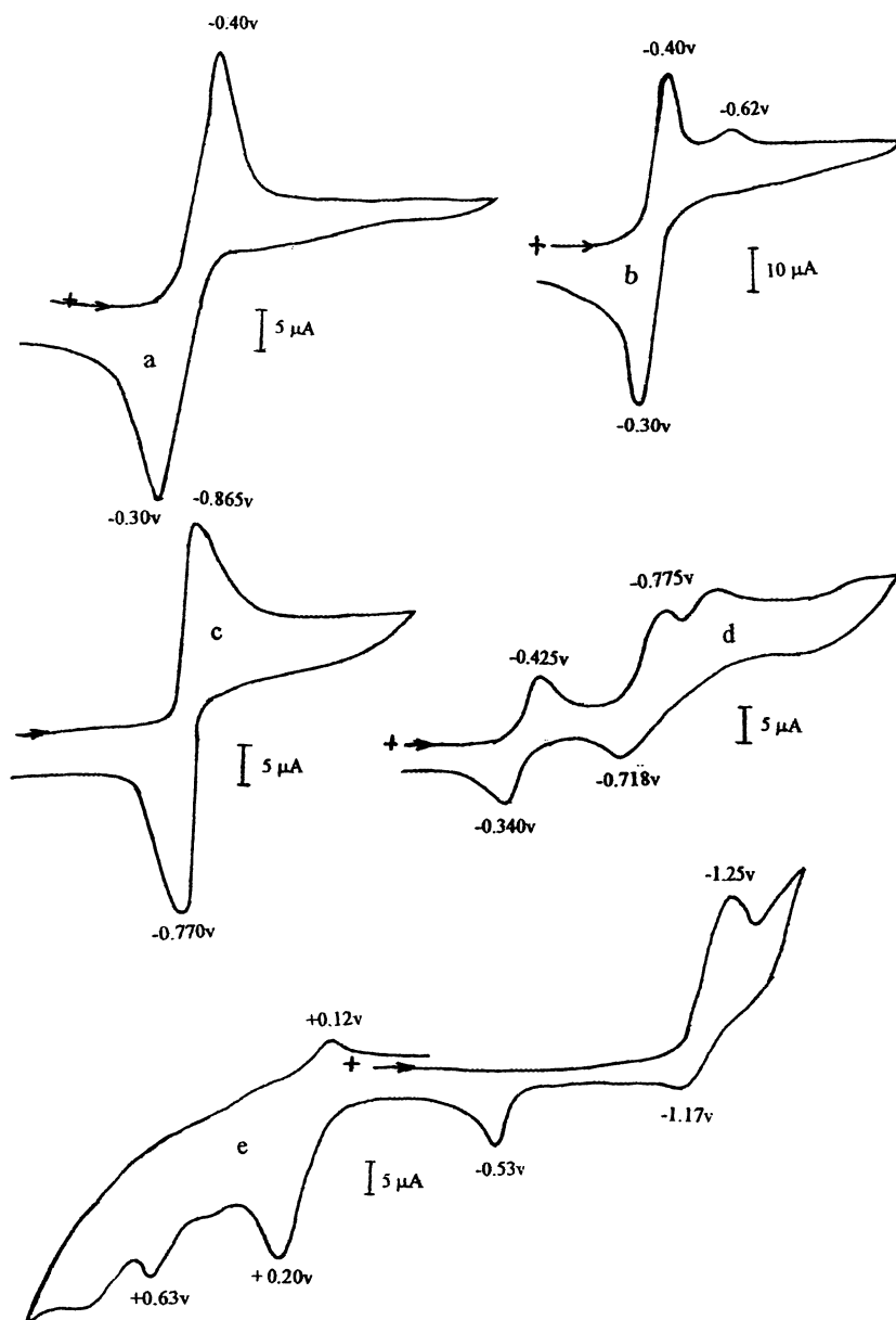
Fig. 5. The voltammograms of 1 , 2 , 3 , 4 and [\text{Mo}_2(\text{SPh})_2(\text{CO})_8] . (a) 1 in \text{Me}_2\text{CO} , v , 100 \text{ mv s}^{-1} , sample concentration, 0.001 \text{ M} ; (b) [\text{Mo}_2(\text{SPh})_2(\text{CO})_8] in \text{Me}_2\text{CO} , v , 100 \text{ mv s}^{-1} , sample concentration, 0.001 \text{ M} ; (c) 2 in \text{Me}_2\text{CO} , v , 100 \text{ mv s}^{-1} , sample concentration, 0.001 \text{ M} ; (d) 4 in \text{Me}_2\text{CO} , v , 100 \text{ mv s}^{-1} , sample concentration, 0.001 \text{ M} ; (e) 3 in \text{Me}_2\text{CO} , v , 100 \text{ mv s}^{-1} , sample concentration, 0.001 \text{ M} .
