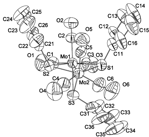
Fig. 2. The structure of the anion of [\text{Et}_4\text{N}][\text{Mo}_2(\text{SPh})_3(\text{CO})_6] ( 2 ).
