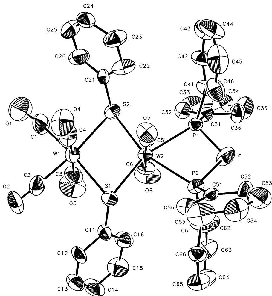
Fig. 4. The structure of [\text{W}_2(\text{SPh})_2(\text{CO})_6\text{DPPM}] ( 4 ).
