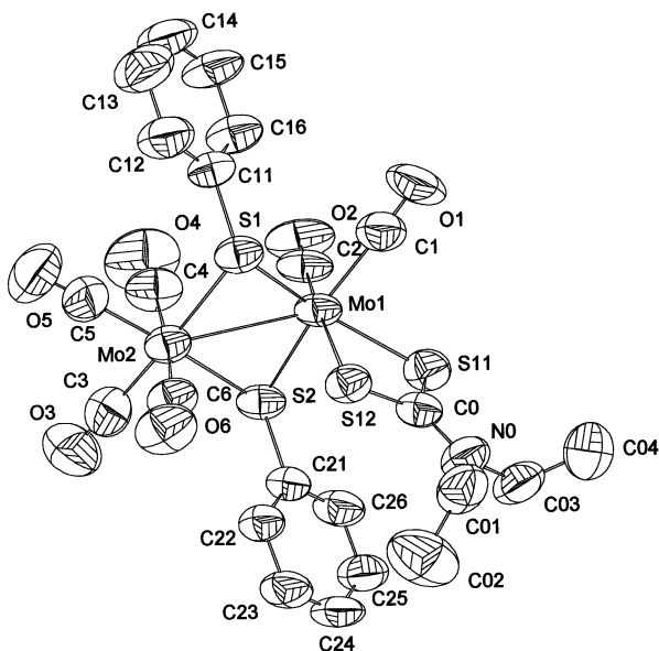
Fig. 3. The structure of the anion of [\text{Bu}_4\text{N}][\text{Mo}_2(\text{SPh})_2(\text{CO})_6-(\text{S}_2\text{CNEt}_2)] ( 3 ).
