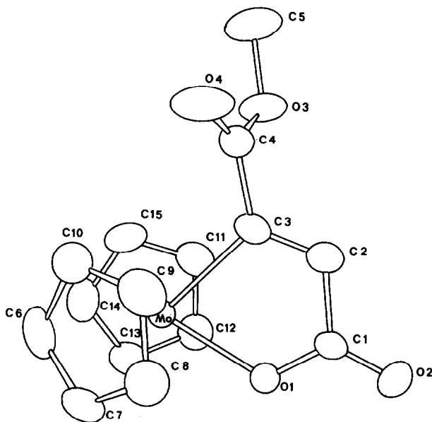
Fig. 3. ORTEP drawing of the organometallic molecule (\eta^5\text{-C}_5\text{H}_5)_2\text{MoOC(O)CH=CHCO}_2\text{CH}_3 in IV showing the atom labelling scheme.
