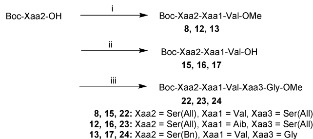
Scheme 4 Reagents and conditions: 22 : (i) 6 , EDC, HOBT, DIPEA, DMF, 0 °C→rt, 22 h, 94%; (ii) LiOH, THF/H 2 O (2:1), 0 °C, 3 h, 71%; (iii) 20 , EDC, HOBT, DIPEA, CH 2 Cl 2 , 0 °C→rt, 16 h, 89%; 23 : (i) 7 , EDC, HOBT, DIPEA, DMF, 0 °C→rt, 22 h, 78% (sum of diastereomers); (ii) LiOH, THF/H 2 O (2:1), 0 °C, 3 h, 88%; (iii) 20 , EDC, HOBT, DIPEA, CH 2 Cl 2 , 0 °C→rt, 27 h, 73%; 24 : (i) 6 , EDC, HOBT, DIPEA, DMF, 0 °C→rt, overnight, 95%; (ii) LiOH, THF/H 2 O (2:1), 0 °C, 3 h, 42%; (iii) 21 , EDC, HOBT, DIPEA, CH 2 Cl 2 , 0 °C→rt, 24 h, 78%.
