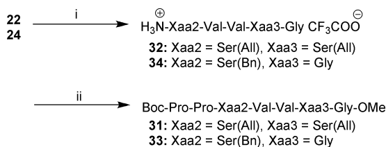
Scheme 5 Reagents and conditions: 33 : (i) TFA, \text{CH}_2\text{Cl}_2 , rt, 1 h 30 min, 92%; (ii) 2 , EDC, HOBt, \text{CH}_2\text{Cl}_2 , 0^\circ\text{C} \rightarrow \text{rt} , 23 h, 78%; 31 : (i) TFA, \text{CH}_2\text{Cl}_2 , rt, 1 h 30 min, 96%; (ii) 2 , EDC, HOBt, DIPEA, \text{CH}_2\text{Cl}_2 , rt, 21 h, 73%.
