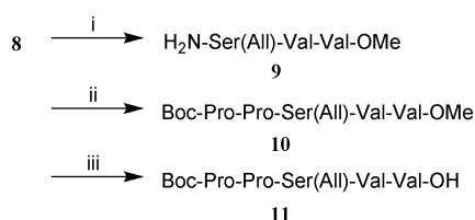
Scheme 2 Reagents and conditions: (i) a. HCOOH, rt, 9 h; b. K 2 CO 3 , H 2 O, 82%; (ii) 2, EDC, HOBT, DIPEA, DMF, 0 °C→rt, overnight, 93%; (iii) NaOH, MeOH/H 2 O (2:1), rt, 8 h.
