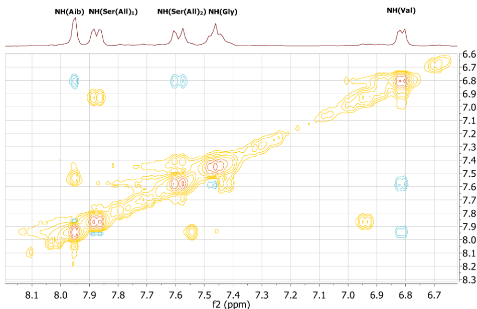
Fig. 5 Partial ROESY spectrum of 30 displaying \text{NH}(i) \rightarrow \text{NH}(i+1) ROEs.
