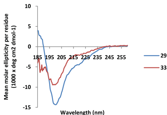
Fig. 4 CD spectra of the heptapeptides 29 and 33 in H 2 O/MeOH (39:1).
