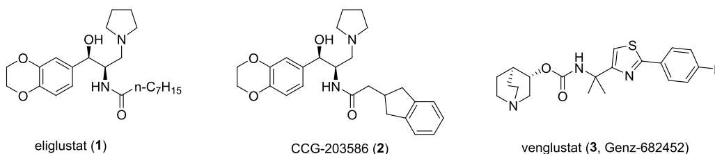
Figure 1. Lead glucosylceramide synthase inhibitors.
