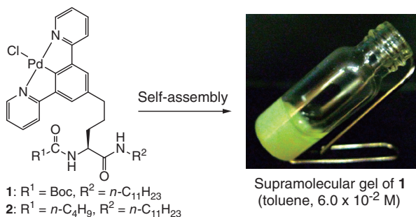
Scheme 1. Supramolecular gel formation of NCN-pincer Pd-complex-bound norvaline derivatives.
