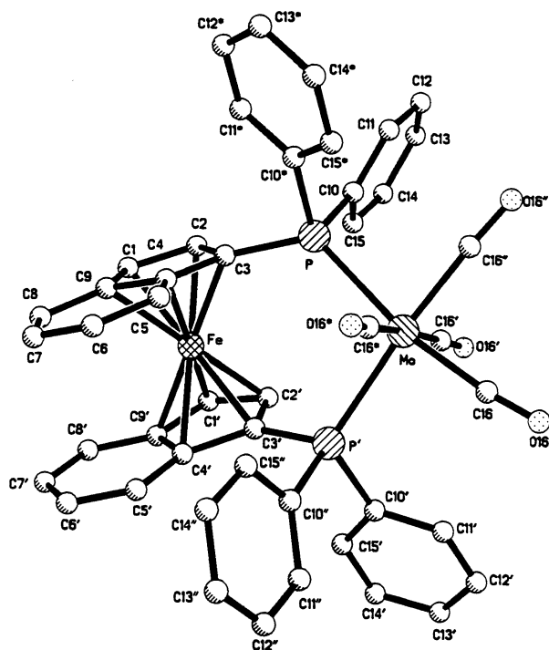
Fig. 2. Thermal ellipsoid plot of 5a .
