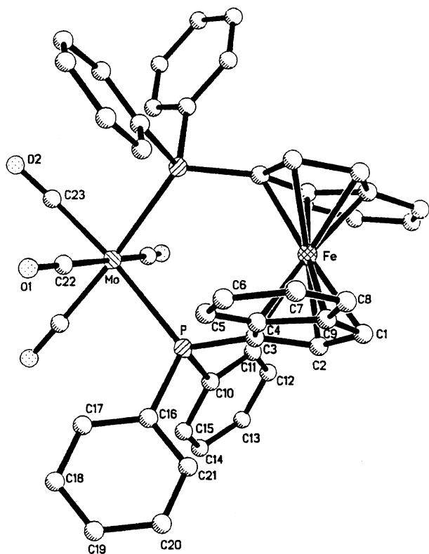
Fig. 4. Thermal ellipsoid plot of 5b .
