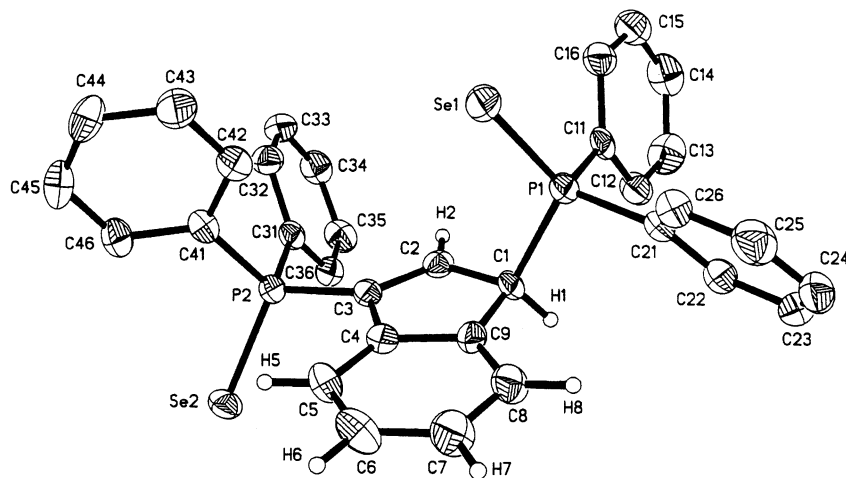
Fig. 1. Thermal ellipsoid plot of one molecule of 2 .
