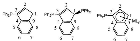
Fig. 5. The adopted atom labelling scheme for the phosphino-indene and -indenyl compounds.
