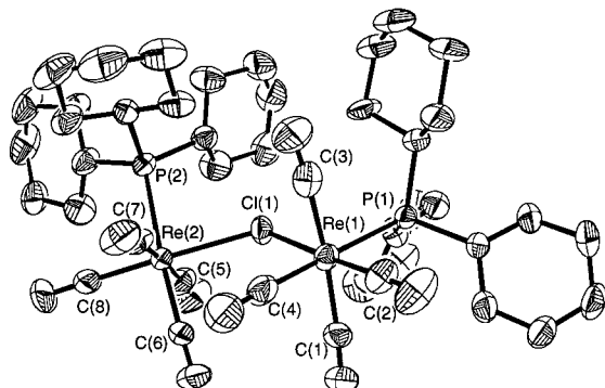
Figure 7. ORTEP diagram for \{[cis-Re(CO)_4(PCy_3)]_2(\mu-Cl)\}\{BAR_F\} , 5c ; BAR_F not shown (50% probability ellipsoids).
