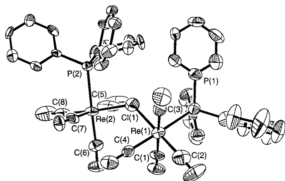
Figure 6. ORTEP diagram for \{[cis-Re(CO)_4(PPh_3)]_2(\mu-Cl)\}\{BAR_F\} , 5a ; BAR_F not shown (50% probability ellipsoids).
