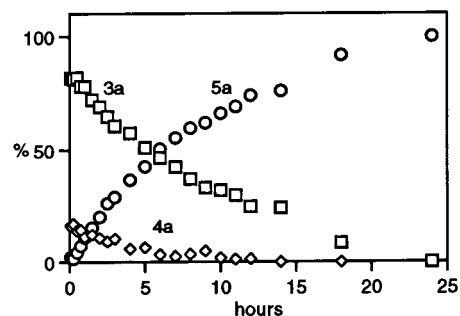
Figure 5. Decomposition of 3a in CD_2Cl_2 solution, 20 °C, monitored by integration of ^{31}P\{^1H\} signals.
