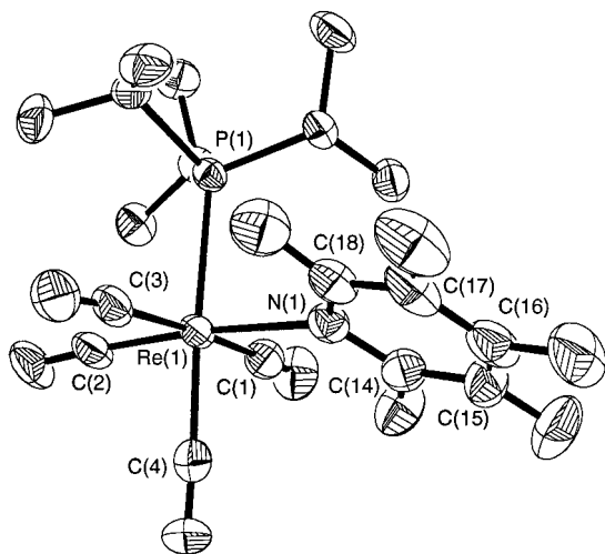
Figure 8. ORTEP diagram for [cis\text{-Re(CO)}_4(\text{P}^i\text{Pr}_3)(\text{NC}_5\text{F}_5)][\text{BARf}] , 6 ; \text{BARf} not shown (50% probability ellipsoids).
