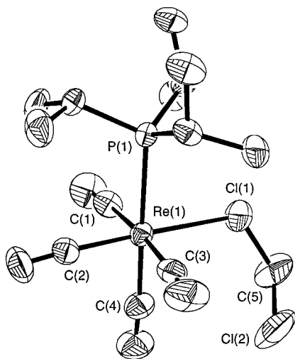
Figure 4. ORTEP diagram for [cis-Re(CO)_4(PiPr_3)(ClCH_2Cl)][BAR_f] , 4b ; BAR_f not shown (50% probability ellipsoids).
