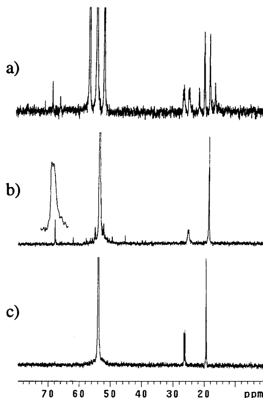
Figure 3. ^{13}\text{C} NMR spectra for [\text{cis-Re}(\text{CO})_4(\text{P}'\text{Pr}_3)(\text{ClCH}_2\text{Cl})][\text{BAR}_\text{F}] , 4b , in \text{CH}_2\text{Cl}_2 solution. (a) ^{13}\text{C} , -80^\circ\text{C} ; (b) ^{13}\text{C}\{^1\text{H}\} , -80^\circ\text{C} ; (c) ^{13}\text{C}\{^1\text{H}\} , 20^\circ\text{C} .
