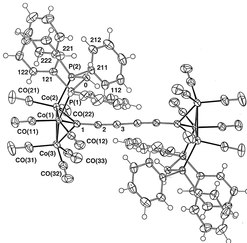
Fig. 1. Plot of a molecule of \{Co_3(\mu\text{-dppm})(CO)_7\}_2\{\mu_3\text{-}\mu_3\text{-C(C}\equiv\text{C)}_2\text{C}\} (1).
