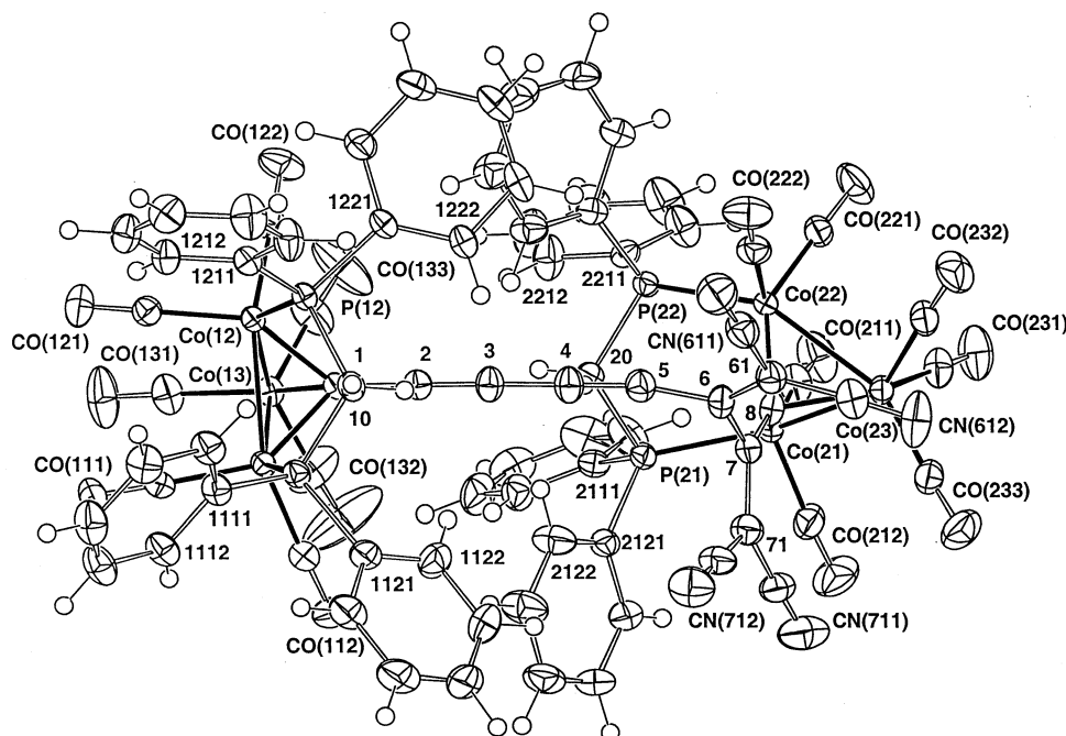
Fig. 3. Plot of a molecule of \{\text{Co}_3(\mu\text{-dppm})(\text{CO})_7\}_2\{\mu_3;\mu_3\text{-C}(\text{C}\equiv\text{C})_2\text{C}[\text{C}(\text{CN})_2]\text{C}[\text{C}(\text{CN})_2]\text{C}\} ( 4 ).
