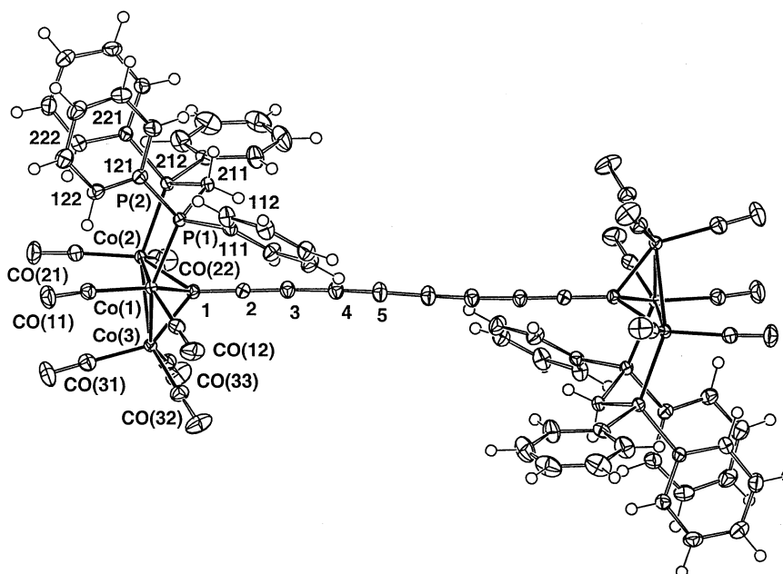
Fig. 2. Plot of a molecule of \{Co_3(\mu\text{-dppm})(CO)_7\}_2\{\mu_3\text{-}\mu_3\text{-C(C}\equiv\text{C)}_4\text{C}\} (3).
