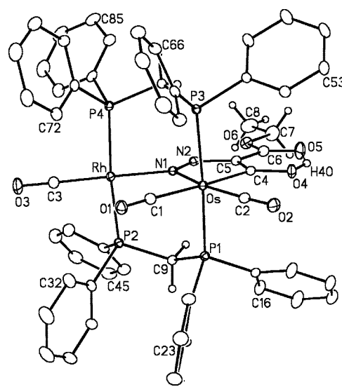
Figure 1. Perspective view of the [\text{RhOs}(\text{CO})_3\{\mu\text{-}\eta^1\text{-}\eta^1\text{-N=NC}(\text{CO})\text{CO}_2\text{Et}\}(\text{dppm})_2]^+ complex cation of compound 8 , showing the atom-labelling scheme. Non-hydrogen atoms are represented by Gaussian ellipsoids at the 20% probability level. Hydrogen atoms are shown with arbitrarily small thermal parameters except for phenyl hydrogens, which are not shown.
