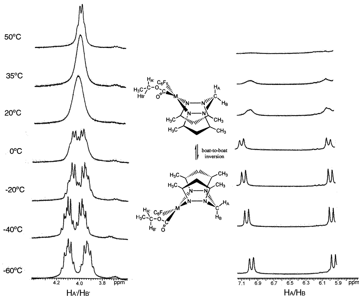
Figure 1. Variable-temperature ^1\text{H} NMR spectra of [\text{Pd}\{\text{CH}_2(\text{C}_3\text{HMe}_2\text{N}_2)_2\}(\text{C}_6\text{F}_5)\{\text{C}(\text{O})\text{OEt}\}] in the C–CH 2 –O (left) and N–CH 2 –N (right) regions, and the boat-to-boat inversion of the metallacycle \text{Pd}(\text{N}–\text{N})_2\text{C} .
