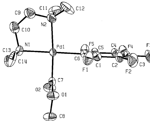
Figure 2. Crystal structure of 8 . Selected bond lengths (Å): Pd–N(1) 2.139(5), Pd–N(2) 2.176(6), Pd–C(6) 2.019(6), Pd–C(7) 1.961(6), C(7)–O(1) 1.329(8), C(7)–O(2) 1.199(8).
