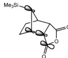
FIGURE 1. Through-bond orbital interactions in 19.
