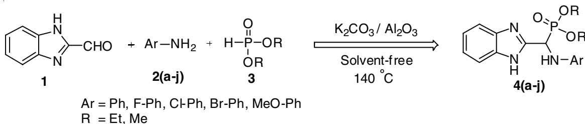
Scheme-I: K_2CO_3/Al_2O_3 catalyzed synthesis of \alpha -aminophosphonates
