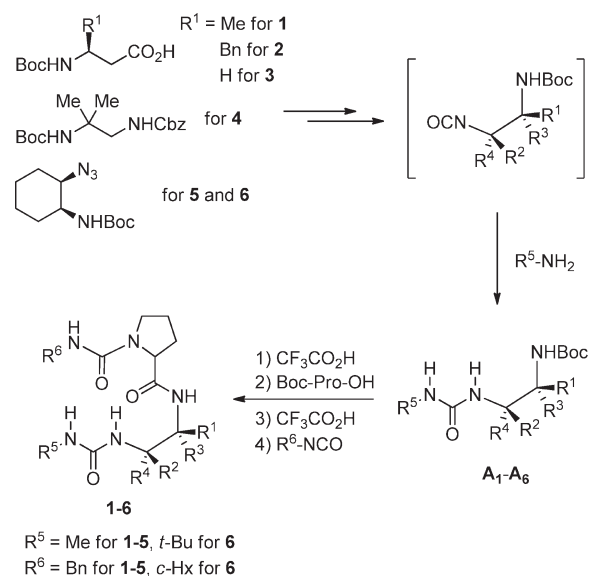
Scheme 1. Summary of the Synthetic Procedures of Nonpeptidic Reverse-Turn Candidates ( 1–6 ) a
