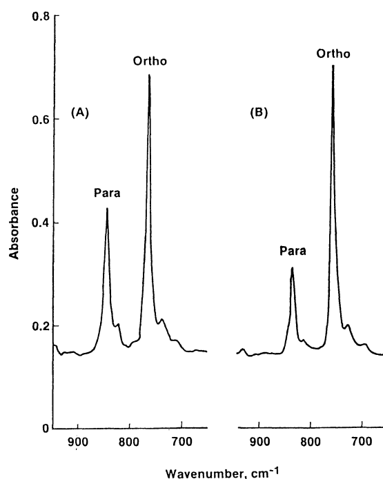
Fig. 1. IR spectra of products from alkylation of phenol with 1-dodecene: (A) 135 °C, ZrO_2 : H_2SO_4 ; (B) 180 °C, H-Mordenite.
